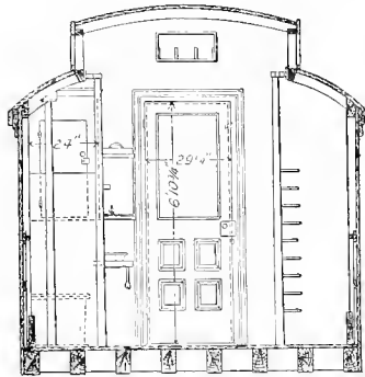
Fig. 611. Transverse Section.
